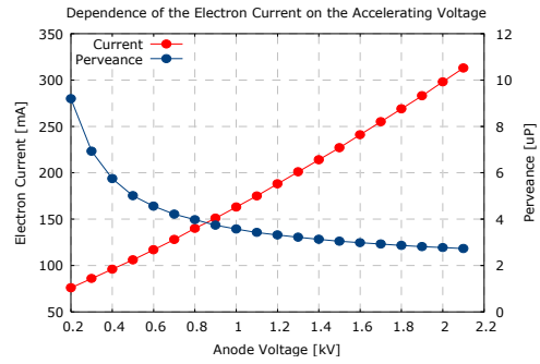
Fig.5 Characteristics of the electron cooler for S-LSR tested at the electron energy of 3.8 keV (corresponding to 7 MeV proton)
