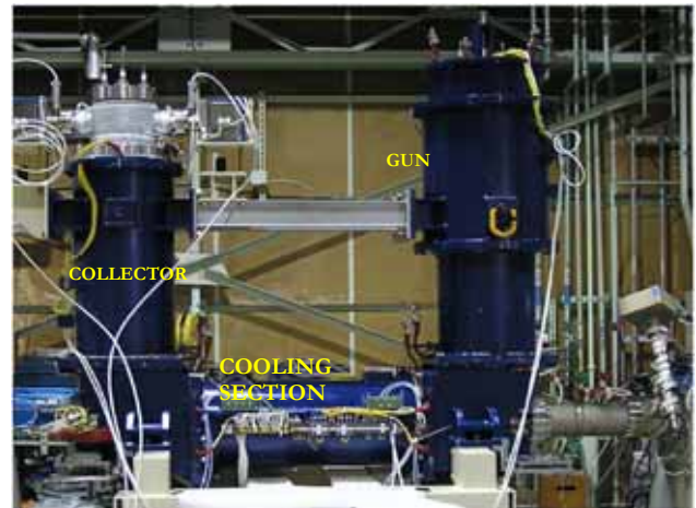
Fig. 3 Fabricated electron cooler for S-LSR.
