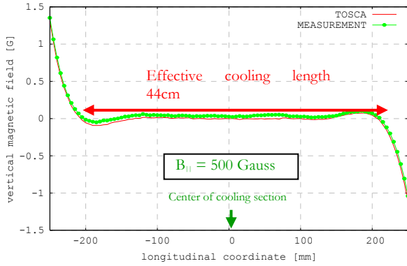
Fig.4 Vertical component of the magnetic field in the cooling section. Measured results are compared with the calculation by the 3 D computer code TOSCA.
