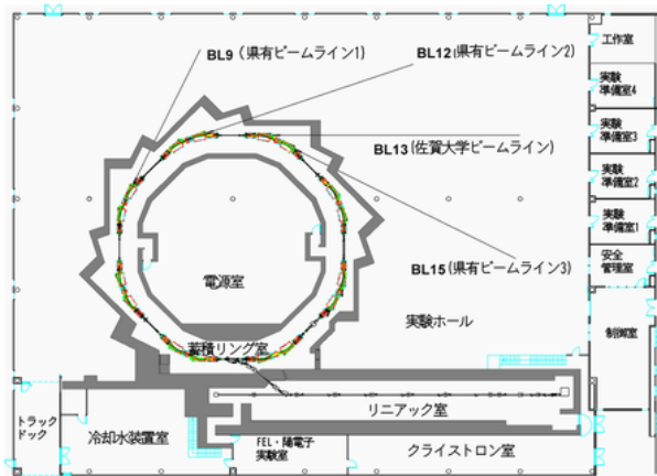
図1 : SAGA Light Source Layout
