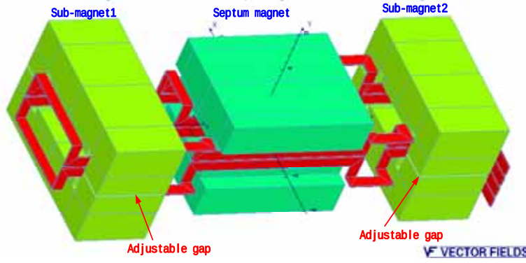
Figure 2: Layout of the septum magnet system
