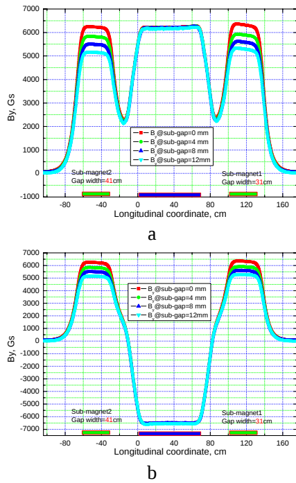
Figure 3: B_y distribution with different sub-bending magnet gap
