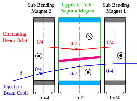
Figure 1: Principle of opposite-field septum magnet
