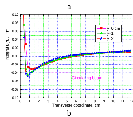
Fig. 6(a,b) The transverse distribution of integral magnetic field
