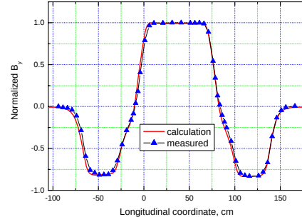
Figure 9: Comparison of measured data and calculation
