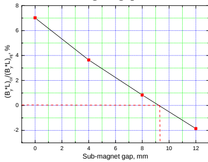
Fig.4 The ratio of integral field (B \cdot L)_{\text{cir}} and integral field (B \cdot L)_{\text{inj}}
