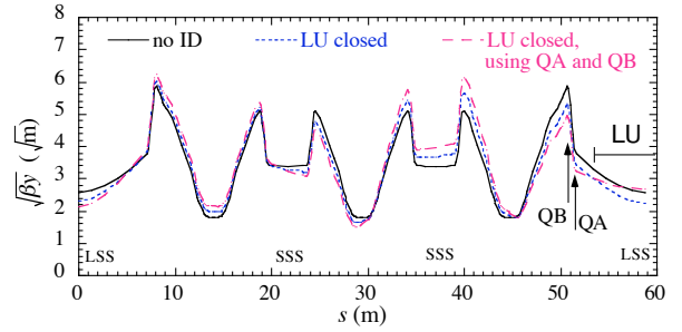
Figure 3 : The effect of LU on the vertical beta functions around the ring. The solid lines show the functions with the gap of LU opened. The dotted line shows the function with the gap of LU closed and no tune shift correction. The broken lines show the beta functions with the gap of LU closed and its tune shift is corrected.
