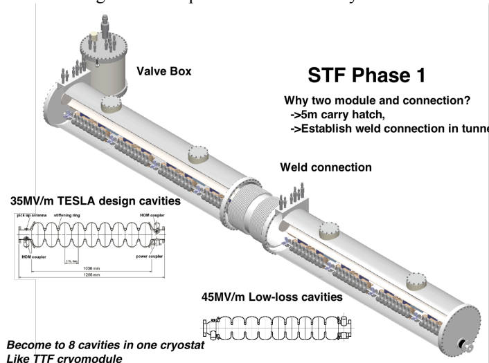
Figure 5 STF phase 1 connected-cryomodule.
