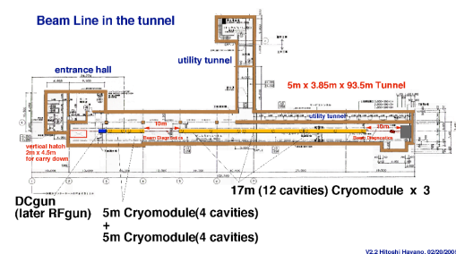
Figure 3 STF tunnel layout plan
