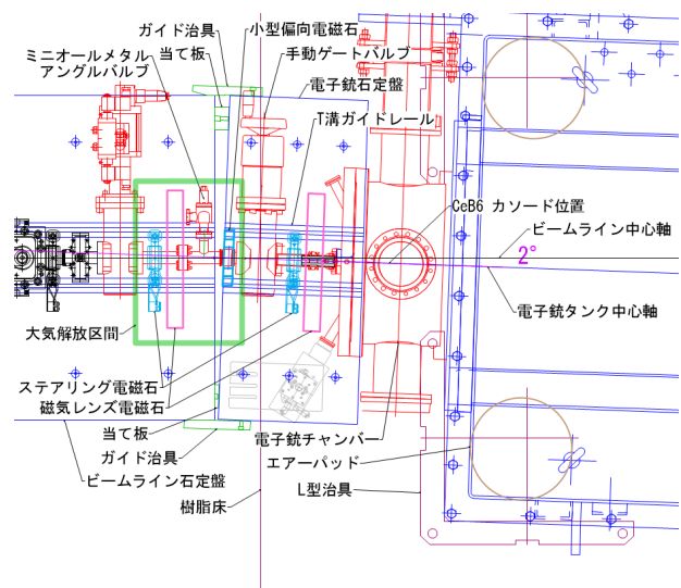
Figure 1: Layout of the modified SACLA electron gun.
