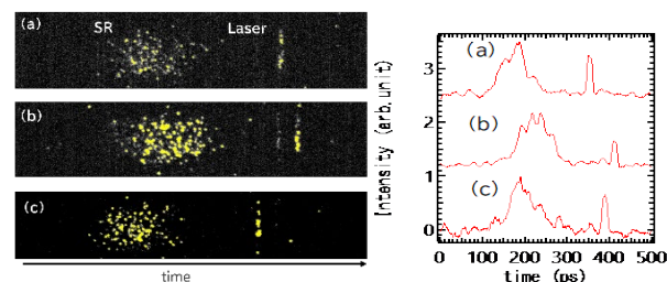
Figure 3: Single-shot-streak profiles of SR and laser pulses.
