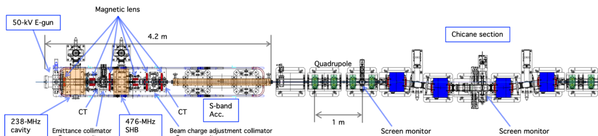
Figure 1: Layout of 40-MeV injector system and chicane section.
