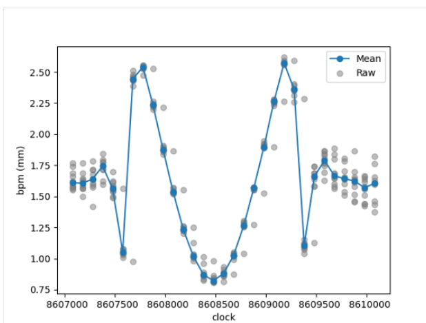
Figure 5: Pulse septum magnet timing optimization. The horizontal axis is a parameter that is proportional to the beam timing. The range corresponds to approximately 6 \mu\text{s} . The vertical axis is the horizontal beam position measured by a BPM downstream of the pulse septum magnet (INJ-BPM2) Gray dots are raw data and blue ones are the mean values of them.
