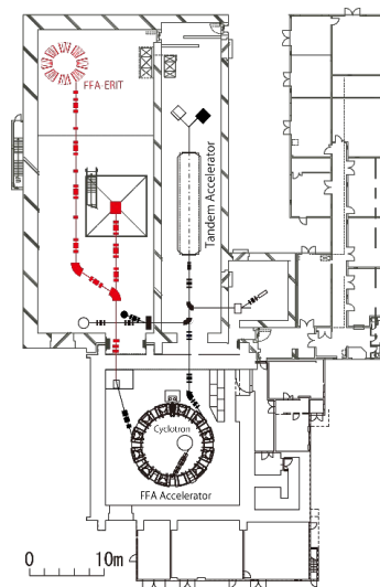
Figure 1: Schematic view of Center for Accelerator and Beam Applied Science in 2023.
