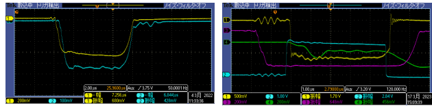
(a) Before renewal, Yellow: No.1 modulator (6 \mu sec) Blue: No.2 modulator (b) After renewal, Purple: No.1 modulator (7 \mu sec)
