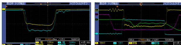
(a) Before renewal, Yellow: No.1 modulator (6 μsec) Blue: No.2 modulator (b) After renewal, Purple: No.1 modulator (7 μsec)
