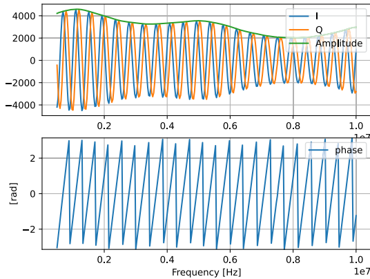
Figure 2: (Top) The measured I and Q and the interpolated ones and (bottom) the phase response calculated from the interpolated I and Q.
