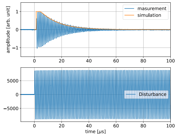
Figure 9: Comparison of measured and simulated step response where P gain = 0.398, I gain = 4e-4 .
