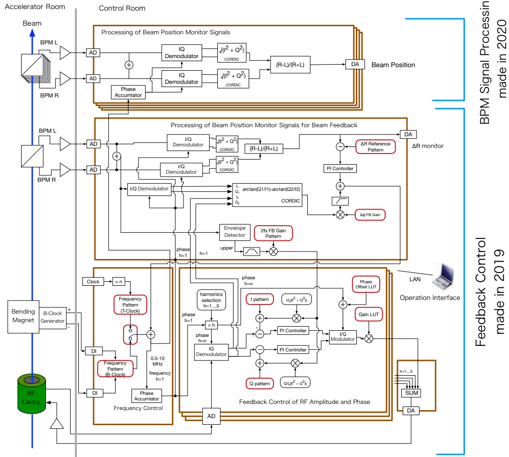
Figure 1: A schematics of New LLRF.
