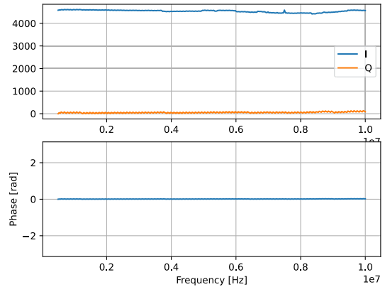
Figure 3: The measured I and Q after setting the gain/phase offset LUT. Amplitude and phase calculated from interpolated I and Q.
