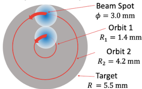
Figure 5: Wobbling scanning schematic on the beam view.
