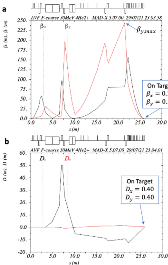
Figure 3: a : Beam oscillation through the beamline b : Beam dispersion.
