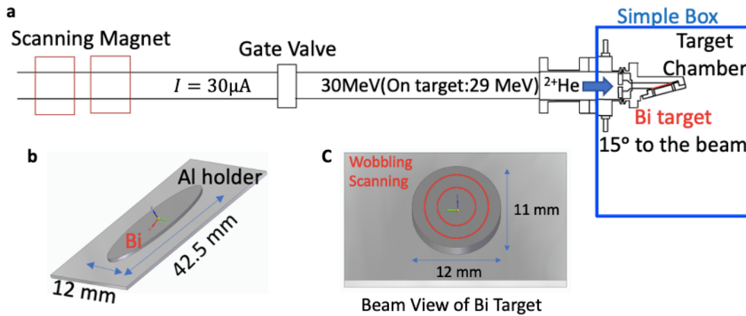
Figure 2: Production of At-211 in RCNP; a : draft of equipment layout in F course b : target size and setup c : scanning schematic on the target.
