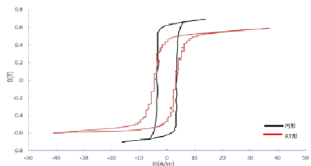
Figure 2: RT core and circular core hysteresis curve.
