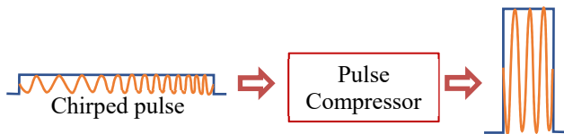
Figure 6: Schematic view of the principle of chirped rf pulse compression.
