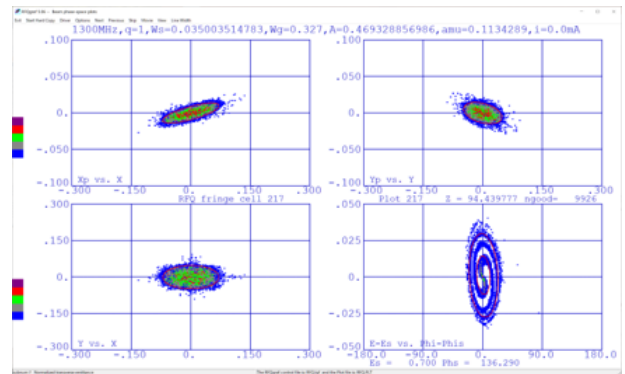
Figure 4: Phase space distribution at the RFQ exit.
