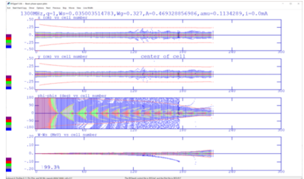
Figure 3: Phase space evolution of the L-band RFQ obtained with RFQGEN.
