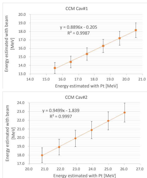
Figure 4: Correlation between energy estimated with beam and energy calibrated for RF pickup.
