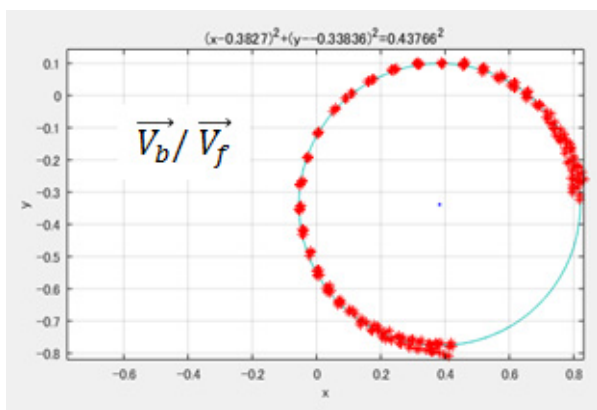
Figure 3: Reflection coefficient obtained by RF input and RF reflected.
