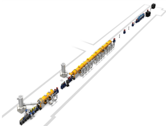
Figure 1: STF-2 accelerator.
