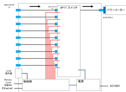
Figure 5: Diagram of RF switching unit.
