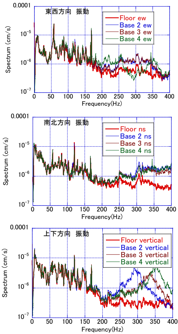
Figure 10: Vibration spectra of floor and Al Base.
