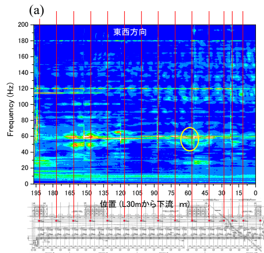
Figure 15: Spectra at both large and small vibration points.
