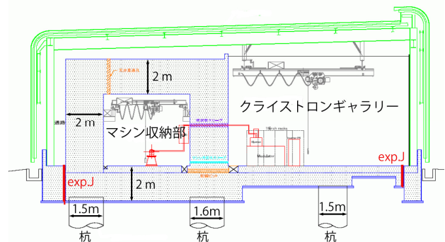
Figure 3: Cross sectional view of accelerator building.
