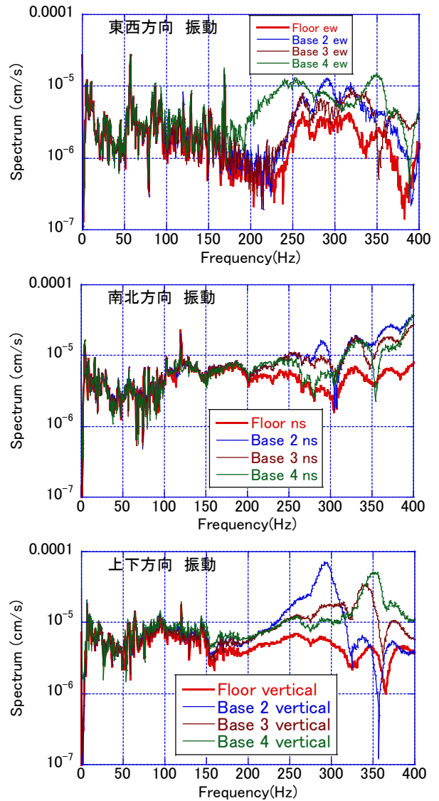
Figure 12: Spectra of floor and Al Base at impulse.
