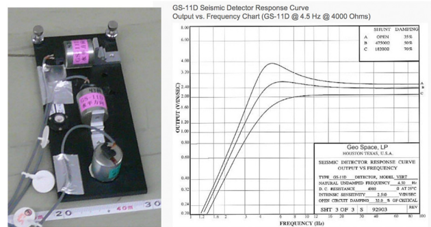
Figure 8: Sensors Geophone (GS-11D) on the Al plate and frequency characteristics.
