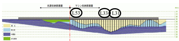
Figure 1: Cross sectional view of SACLA foundation.
