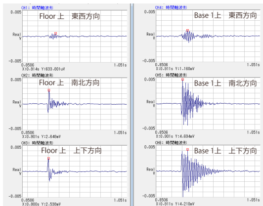
Figure 11: Velocities of floor and Al Base at impulse.
