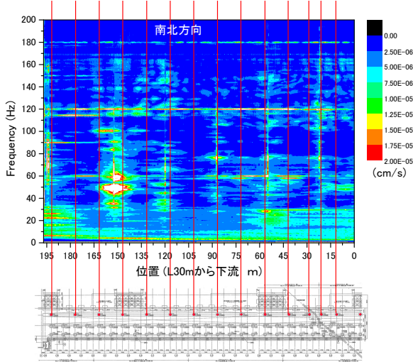
Figure 17: NS vibration spectra and pile positions.
