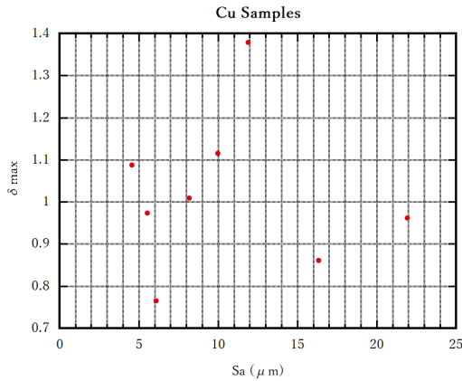
Figure 7: The final \delta_{\text{max}} of copper samples as a function of Sa.
