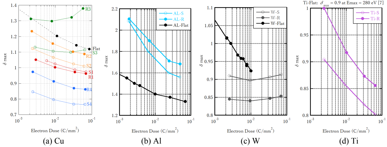
Figure 2: The final \delta_{\max} of (a) Cu, (b) Al, (c) W and (d) Ti samples as a function of electron dose.
