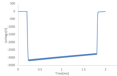
Figure 4: Output voltage at 1/8 shift.
