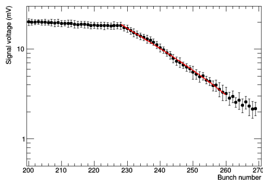
Figure 2: Typical data plot of the averaged signal peaks at the decaying range. The red line is the fitting line with Eq. 1.
