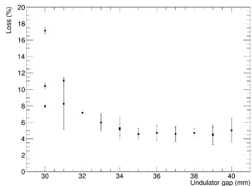
Figure 3: Single round-trip loss for each undulator gap.
