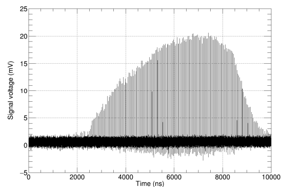
Figure 1: Typical waveform of the FEL pulses measured by the P5 pyroelectric detector.
