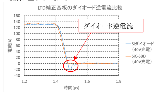
Figure 9: Typical output current waveforms of diodes mounted on the correction circuit.
