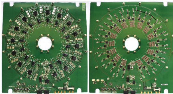
旧補正基板 新補正基板 Figure 7: Photos of the correction circuit.
