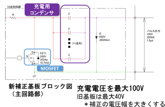
Figure 6: Block diagram of the correction circuit.
