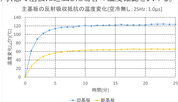
Figure 5: Measurement result of temperature rise of the reflected wave absorber.
