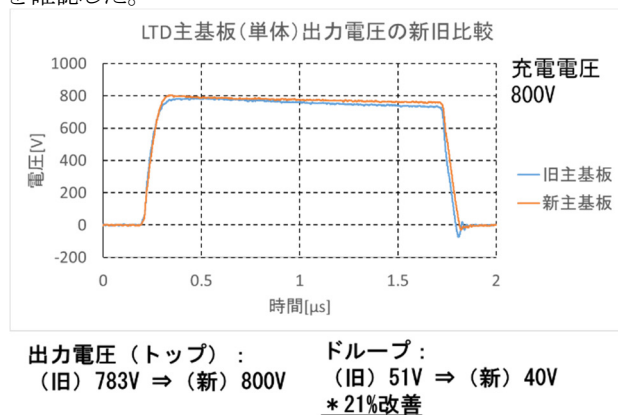
Figure 4: Comparison of output voltages of old and new circuits.
