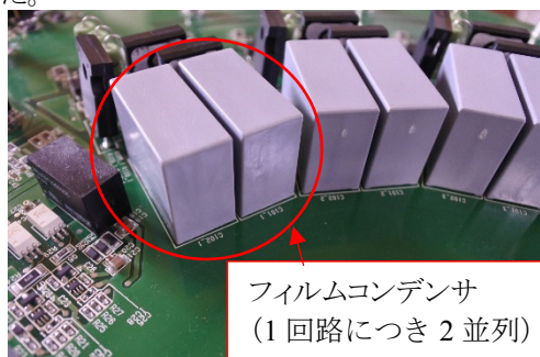
Figure 3: Photo of the film capacitor mounted on a new circuit.
