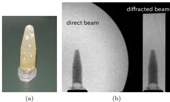
Figure 6: (a) A plastic tube filled with epoxy resin containing \text{SrTiO}_3 fragments. (b) A typical projection image of simultaneous-KES CT.
