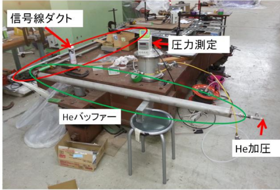
Figure 8: Set up of airtight test
