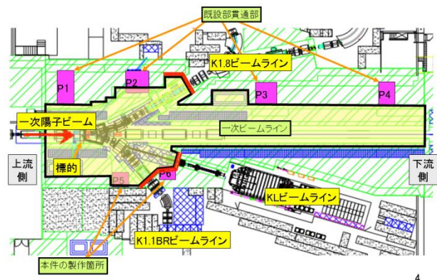
Figure 1: The floor plan of J-PARC Hadron experimental Hall
