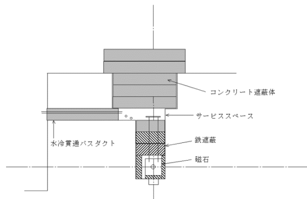
Figure 2: The cross section of the primary beam line at J-PARC Hadron experimental Hall
