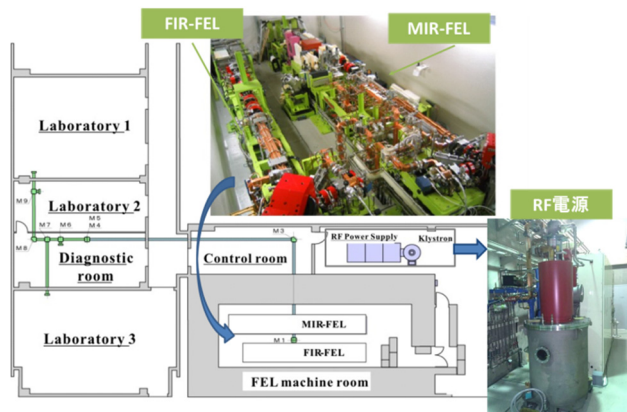
Figure 1: Layout of FEL-TUS.
