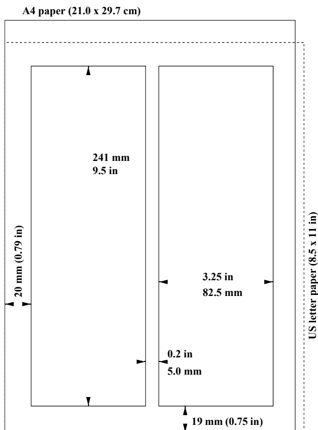
Figure 1: Document layout.
