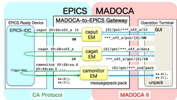
Figure 1: Scheme of MADDOCA-to-EPICS gateway.
