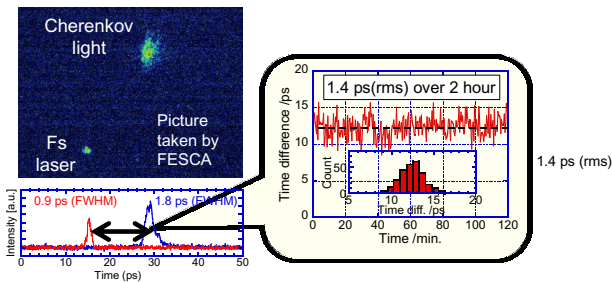
(a) synchronization between fs laser & EB pulse
