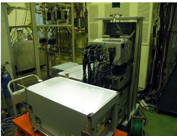
Figure 2: Photo of 3.95 MeV X-ray source based on X-band linac.
