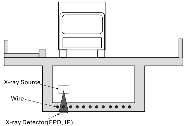
Figure 3: Sectional drawing of NDT for Myoko-bridge.
