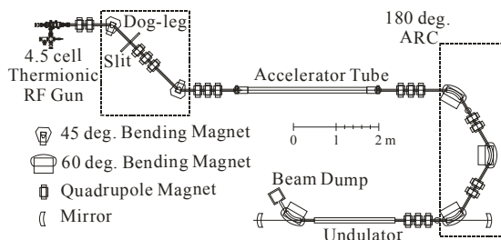
Figure 1: Schematic drawing of KU-FEL accelerator and FEL devices in July 2016.
