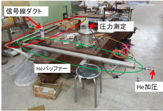
Figure 8: Set up of airtight test
