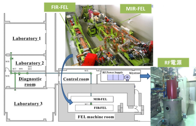
Figure 1: Layout of FEL-TUS.
