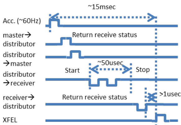
Figure 3: Timing sequence of the tag data supply system.
