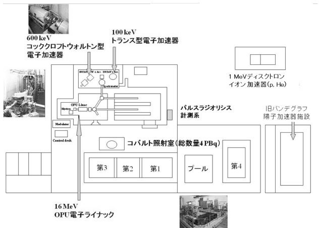
Figure 2: Schematic diagram of the accelerators and the irradiation facilities.
