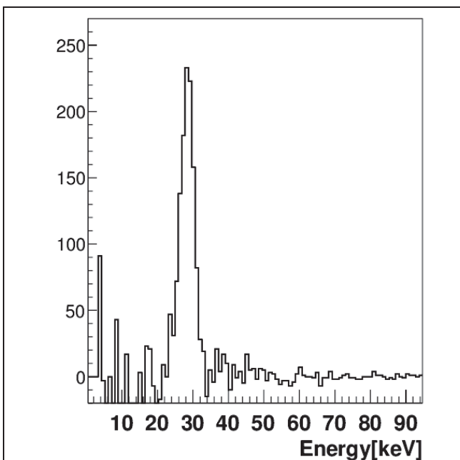
Figure 8 : Detected X-ray spectrum on SOI detector
