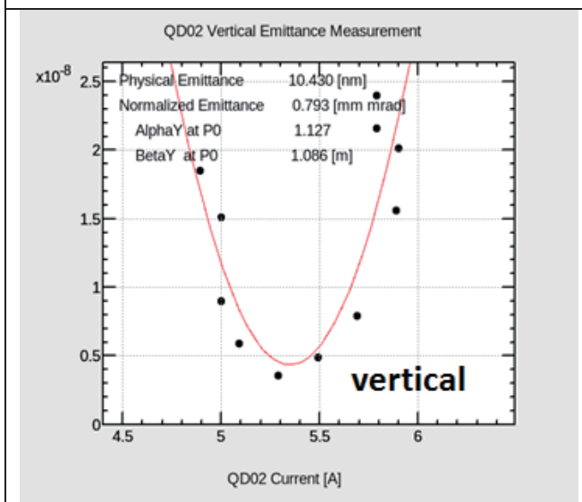
Figure 3 : Emittance measurement results
