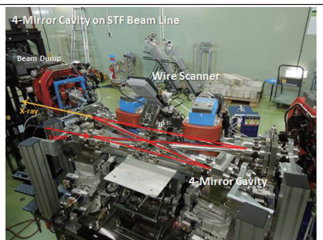
Figure 5 : 4-Mirror optical cavity
