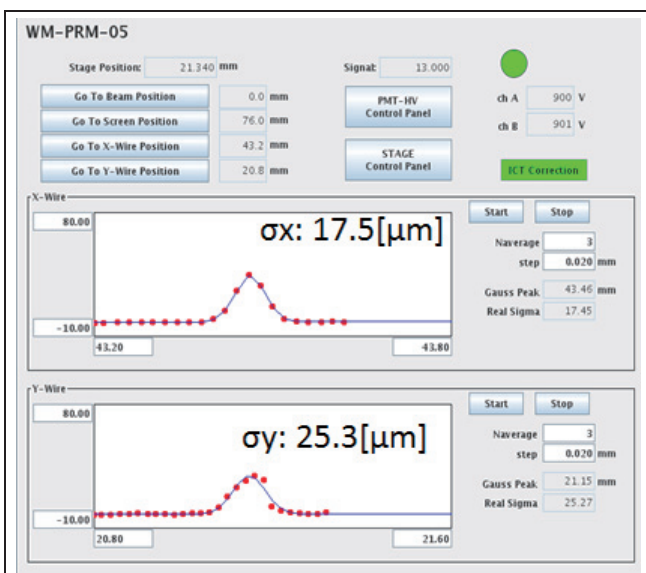
Figure 2 : Typical beam size measured by tungsten wire
