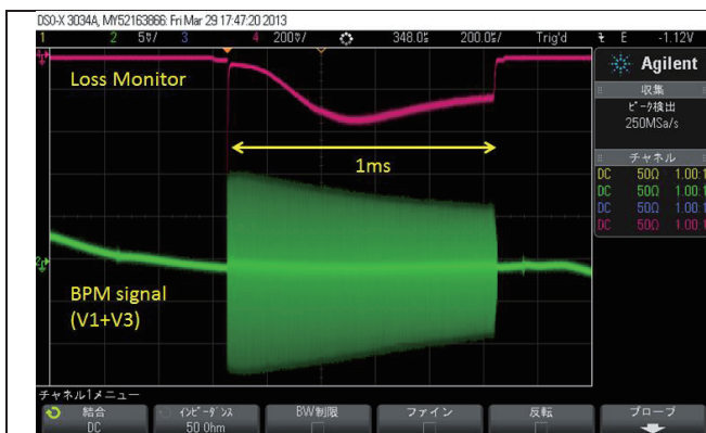
Figure 4 : Achieved 1ms long bunch at STF
